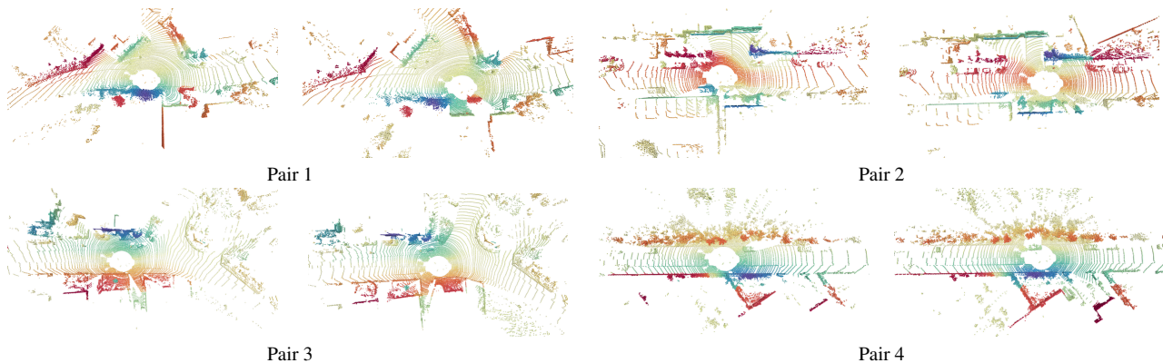
Figure 6: Color-coded FCGF features for pairs of KITTI LIDAR scans that are 10m apart. FCGF features from downsampled LIDAR scans are mapped to a scalar space using t-SNE [33] and colored with the Spectral color map.
