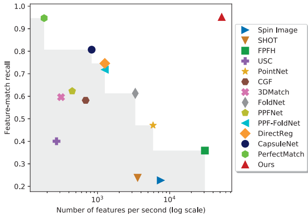
Figure 1: Feature-match recall [6, 7] and speed in log scale on the 3DMatch benchmark [38]. Our approach is the most accurate and the fastest. The gray region shows the Pareto frontier of the prior methods.
